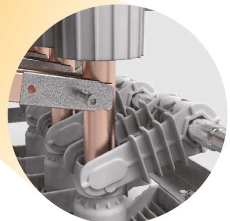
Earthing Switch
